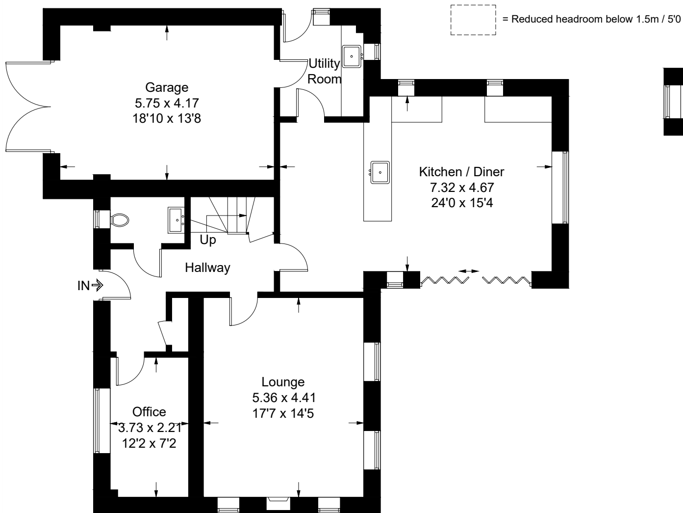
Ground Floor
